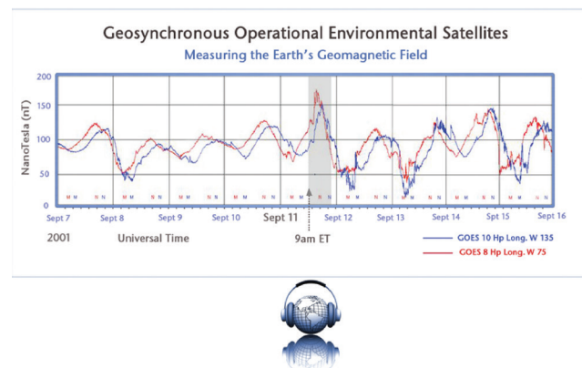
Figure 12: The data recorded from the Geostationary Operational Environmental Satellite 8 and 10 which are in geosynchronous orbit over the east and west coasts of the United States in the days before, during, and after the September 11, 2001, terrorist attacks.
